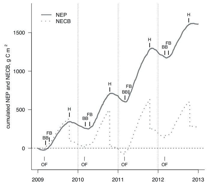
Fig. 5. – Cumulated trend of NEP and NECB ( g C m^{-2} ) during the four monitored years (2009–12). Letters above the NEP line indicate the occurrence of phenological phases (BB = Bud Burst; FB = Full Bloom; H = Fruit Harvest). Letters below NECB line indicate time of fertilization, which introduced organic carbon into the ecosystem (OF = Organic Fertilizer).
