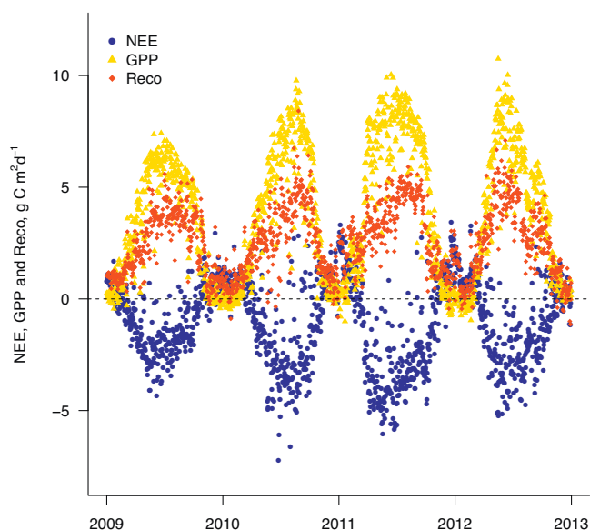
Fig. 2. – Daily values of NEE, GPP, and R_{eco} ( \text{g C m}^{-2} \text{ d}^{-1} ) during the four monitored years (2009–12).
