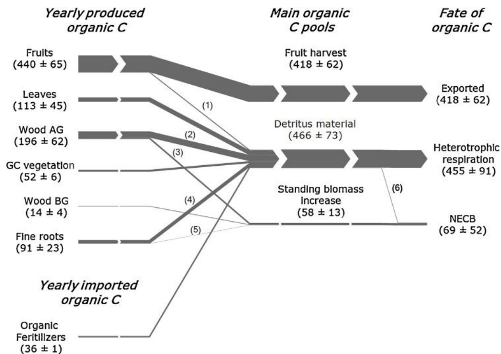
Fig. 6. – Overall scheme of the fate of the carbon made annually available by NPP and by organic fertilizer, with arrow size proportional to observed fluxes. Data are expressed in \text{g C m}^{-2} \text{ year}^{-1} and represent the average of three years (2010–12) and the standard error. On the left side the amount of carbon annually entering the ecosystem through photosynthesis fixation as net primary production (Wood AG and wood BG means aboveground and belowground woody NPP, respectively; GC vegetation indicates the aboveground ground-cover vegetation production of the alley) and through organic fertilization is presented. In the middle part of the scheme the main C pools formed during the vegetative season are shown. On the right side, the fate of the carbon is reported: the apple production is removed from the ecosystem at the end of the season (exported C); the heterotrophic respiration data are calculated by difference between the sum of the data on the left side of the scheme and the sum of NECB and exported C; the NECB represents the average net carbon balance during the measurement period. (1) refers to the dropped fruits ( 22 \pm 3 \text{ g C m}^{-2} \text{ year}^{-1} ); (2) refers to pruning material ( 167 \pm 53 \text{ g C m}^{-2} \text{ d}^{-1} ); (3) is the increment of above ground biomass ( 29 \pm 9 \text{ g C m}^{-2} \text{ d}^{-1} ); (4) fine root turnover ( 87 \pm 28 \text{ g C m}^{-2} \text{ d}^{-1} ); (5) is the increment of fine root standing biomass ( 5 \pm 2 \text{ g C m}^{-2} \text{ d}^{-1} ); (6) is the fraction of detritus material contributing to NECB ( 21 \pm 53 \text{ g C m}^{-2} \text{ d}^{-1} ).
